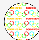
Diffractive microimages of «Olympic Rings» with repeated text «SOCHI 2014» 70 micron high
